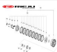
CLUTCH SYSTEM
