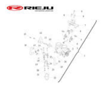
INJECTION BODY
