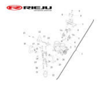
INJECTION BODY
