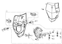
FRONT LIGHT
