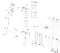
FORK
